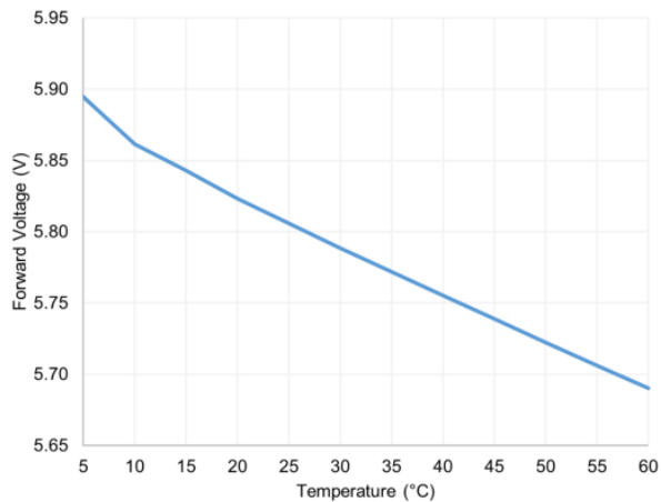
Figure 8. Forward voltage vs temperature (T solder )
