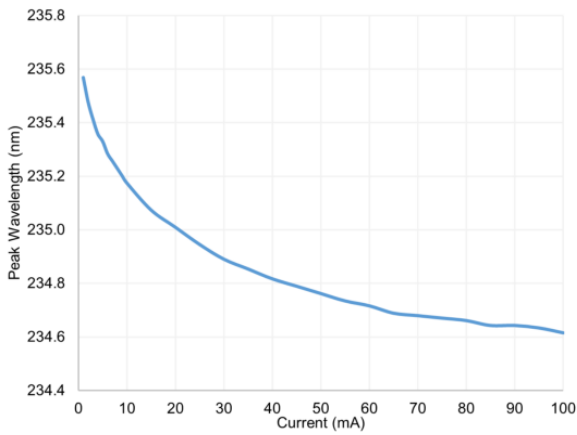
Figure 3. Peak wavelength vs forward current T_A=25\text{ }^\circ\text{C}
